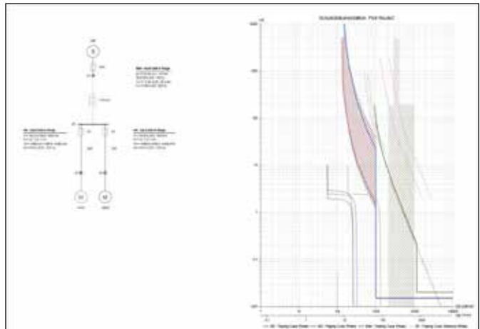
Documentation of a protection path including path in network and its diagram with result data
