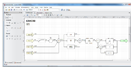
Figure 1: Graphical Model Builder (GMB)
