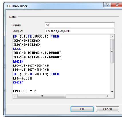
Figure 4: Special user blocks with FORTRAN statements
