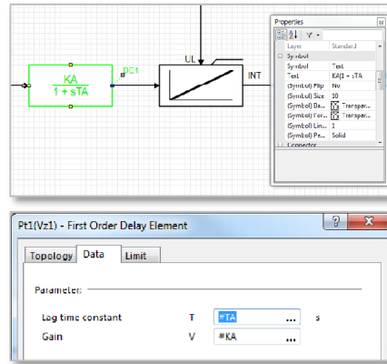
Figure 3: Data input in masks after double clicking
