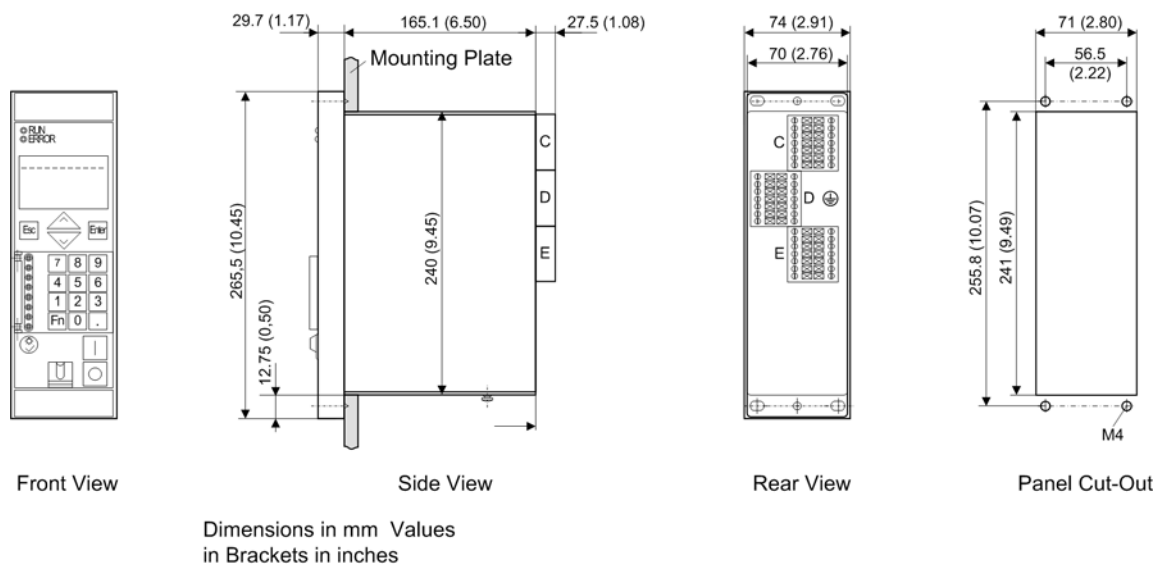
Figure 4-2 Dimensional drawing of a 7RW80 for Panel Flush and Cubicle Mounting (Housing Size 1/6)
