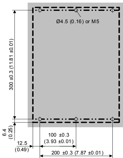
Mounting Holes of Mounting Plate
