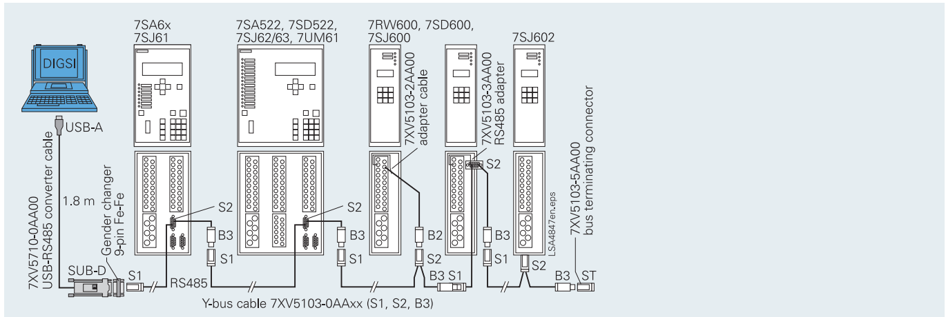
Fig. 13/77 Central operation via the RS485 bus
