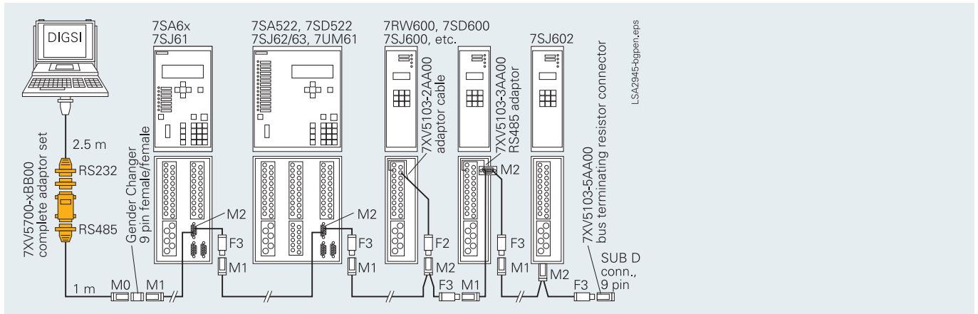
Fig. 13/74 Protection units connected to the RS485 bus
