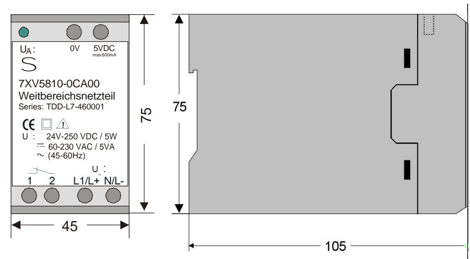
Abb. 4: Dimension Drawings
