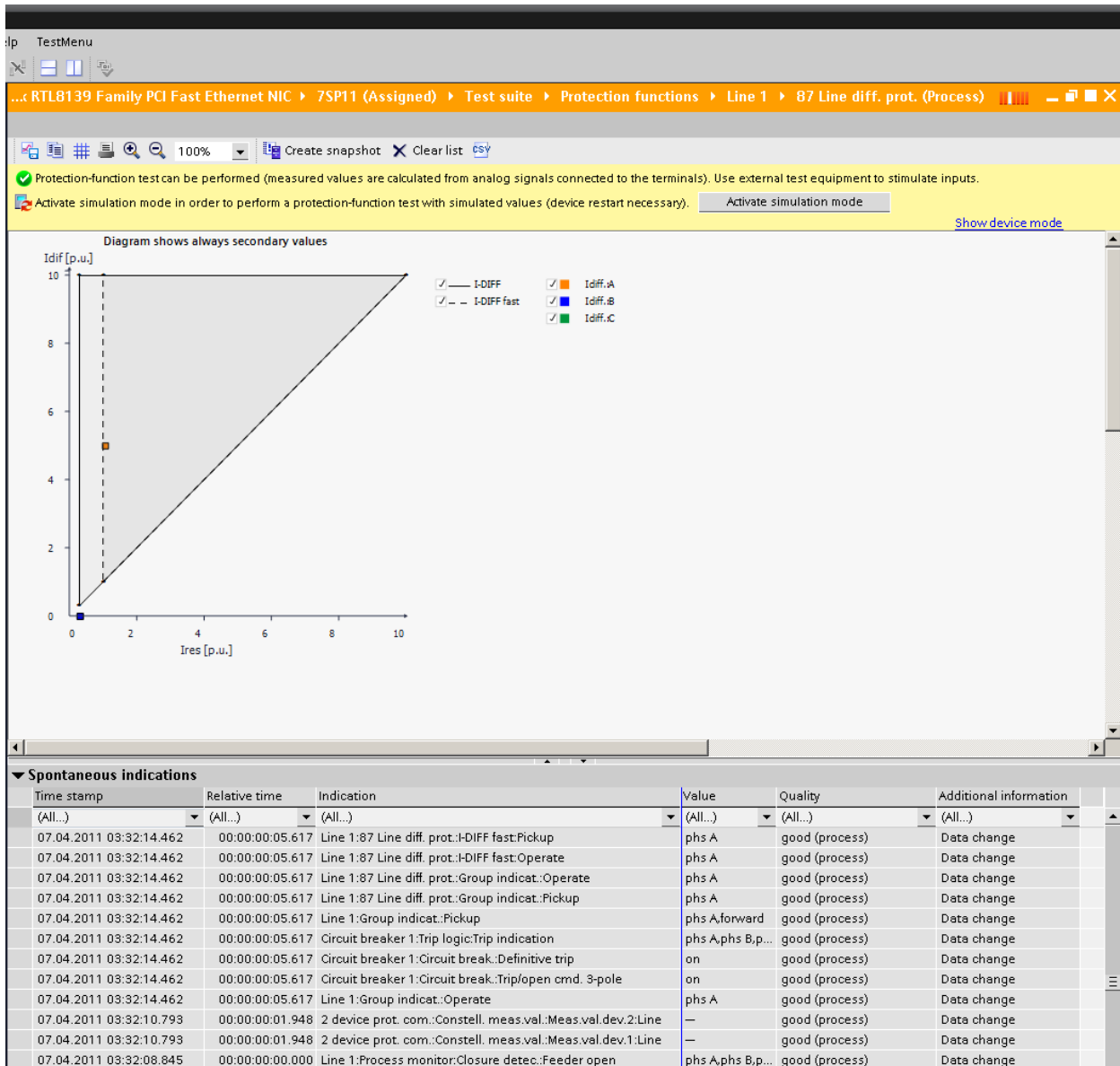
Figure 4: Testing a protection function with a test sequence. Reaction in the tripping characteristic and spontaneous fault indication of the device
