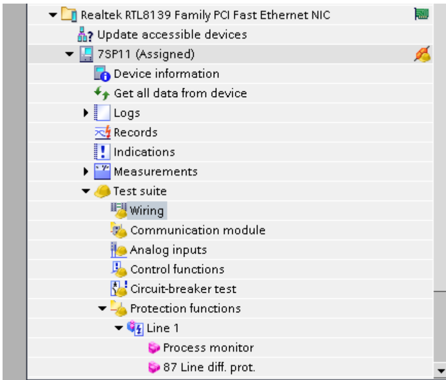
Figure 5: Test editor for the wiring test in DIGSI 5
