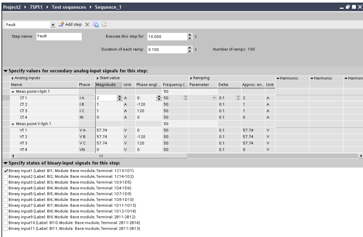
Figure 1: Editor for test sequences in DIGSI 5
