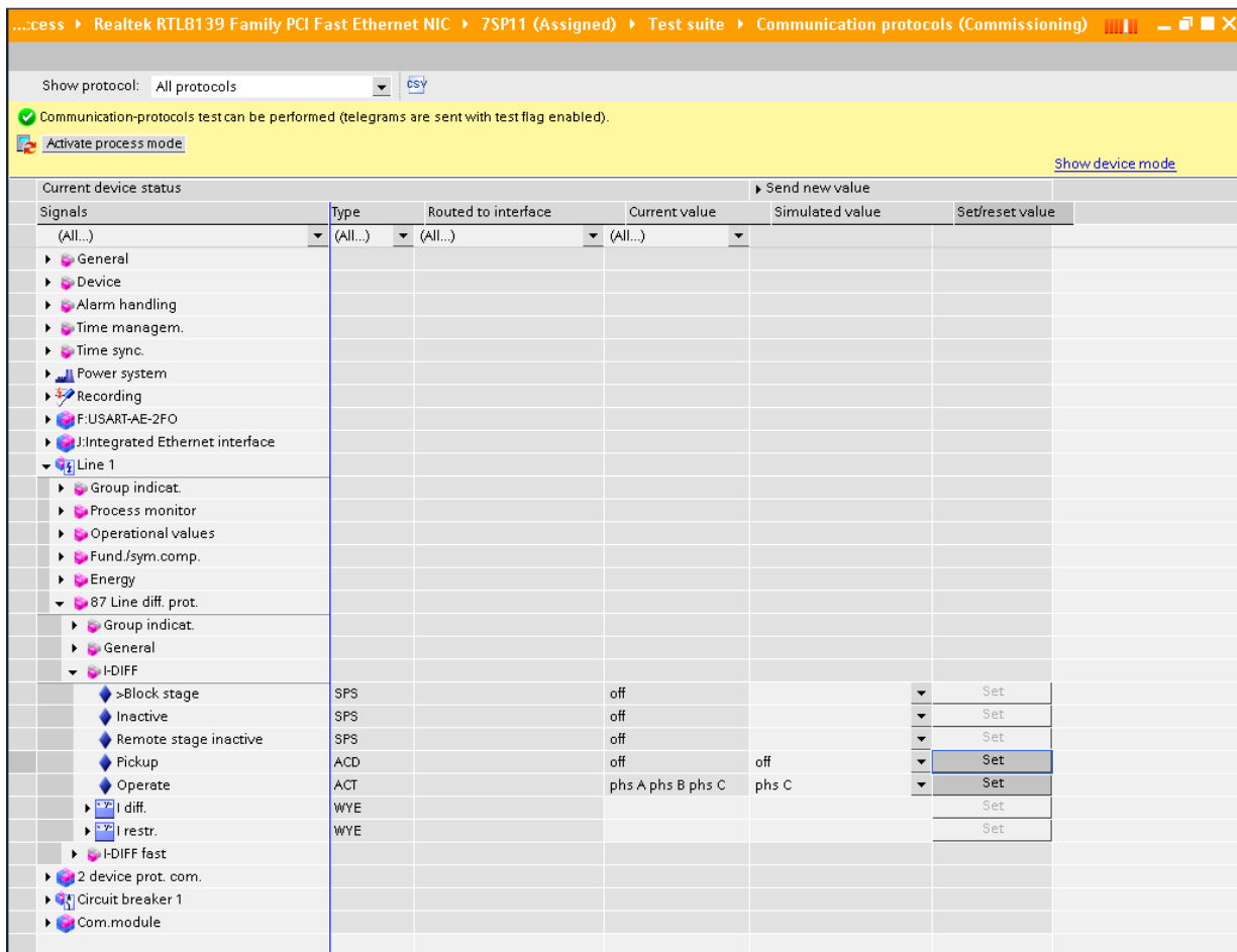
Figure 8: Communication protocol test editor in DIGSI 5
