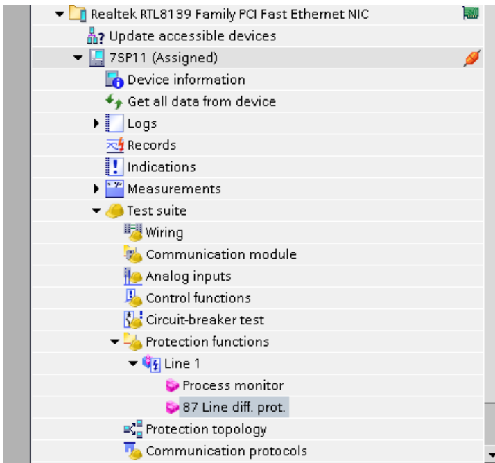
Figure 2: Open the editor for testing protection functions
