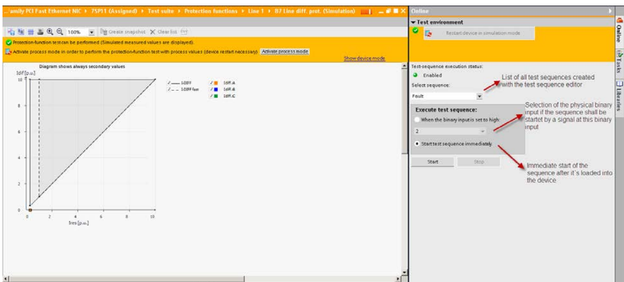
Figure 3: Testing a protection function with a test sequence created by the sequence editor
