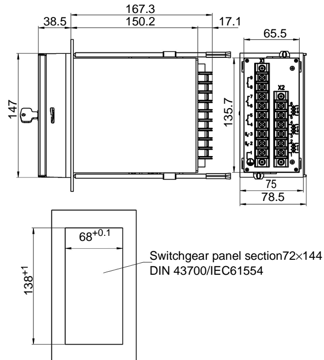
Figure 2-7 Dimensional drawings
