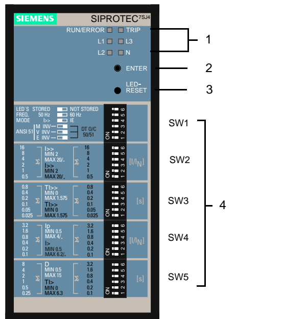
Figure 2-1 Device front of the 7SJ46 with indication and control elements
