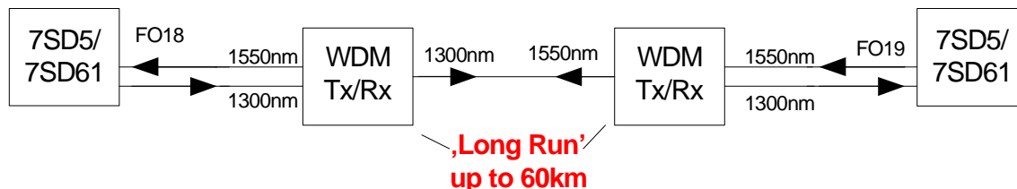
Figure 4: WDM with one PDI and only one optical fibre
