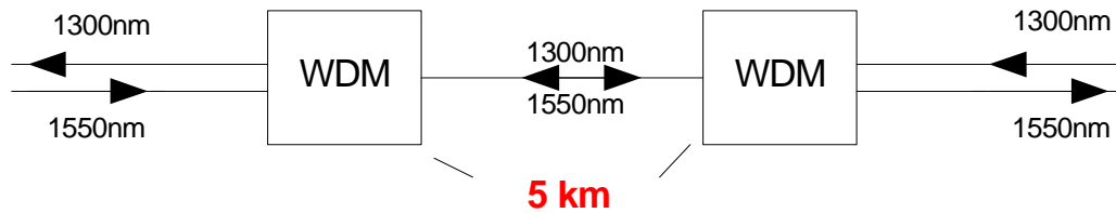
Figure 8: 5 km example using one fibre
