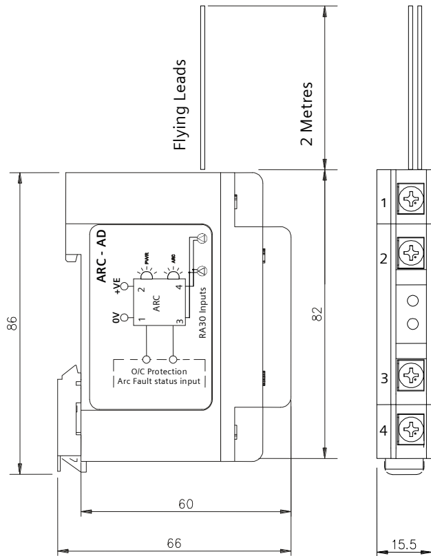
Figure 8: RA23 Module dimensional details
