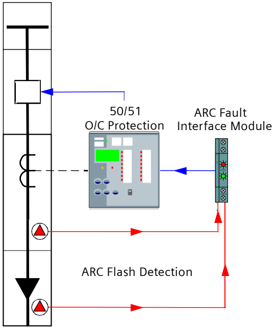
Figure 1: Cable box and CT chamber protection
