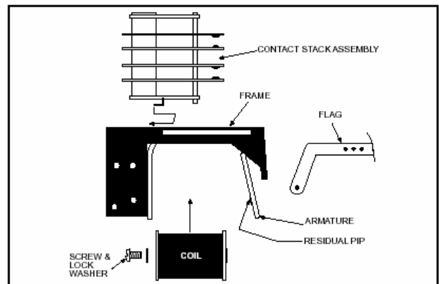
Major component parts of a typical attracted armature relay
