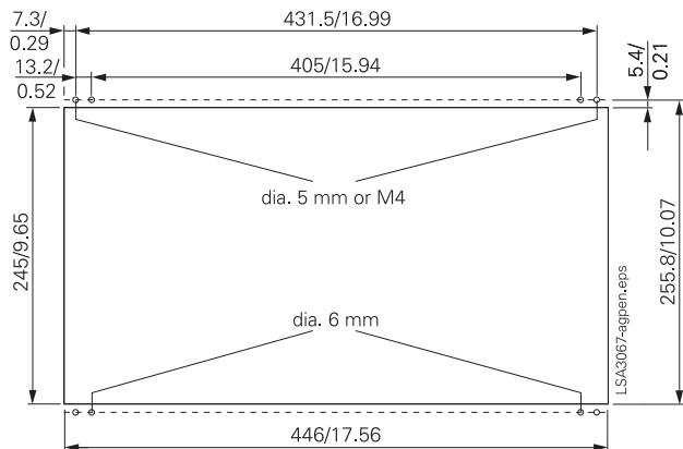
Panel cutout
