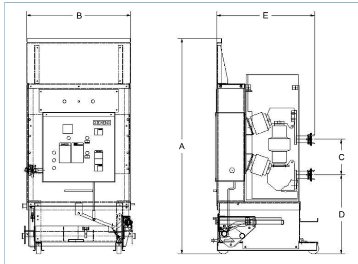
Sample dimensional diagram – HKR
