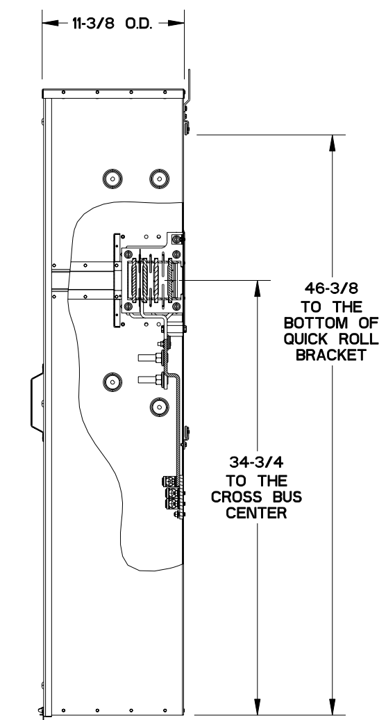
PARTIAL SECTION
