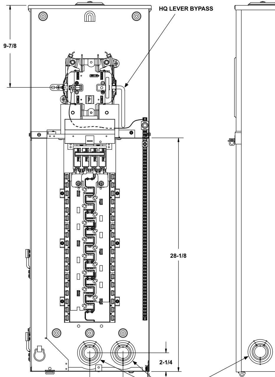
VIEW SHOWN WITH DEADFRONT AND COVERS REMOVED
