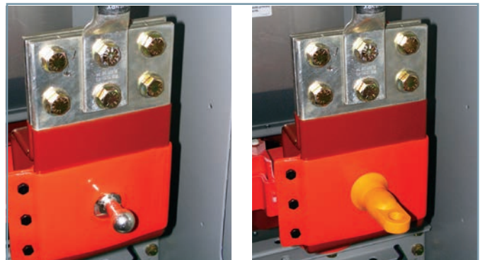
Figure 2: Ball-type ground stud - left with cover removed, right with cover in place
