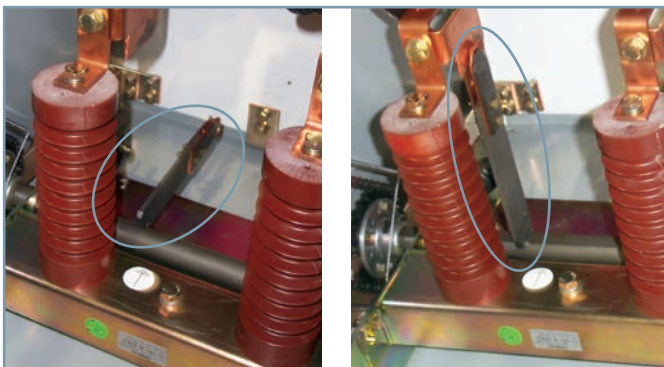
Figure 1: Grounding switch - left in normal (non-grounded) position, right in ground position
