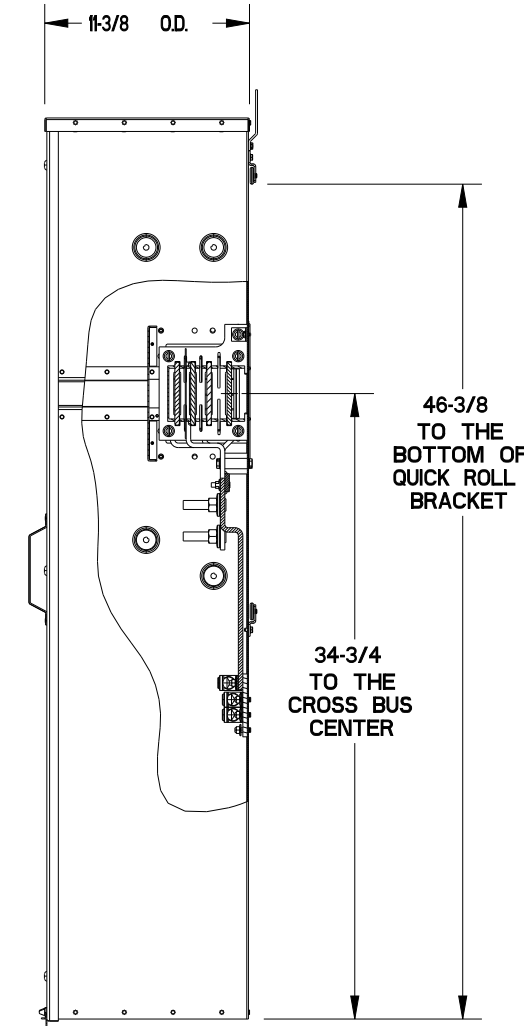
PARTIAL SECTION
