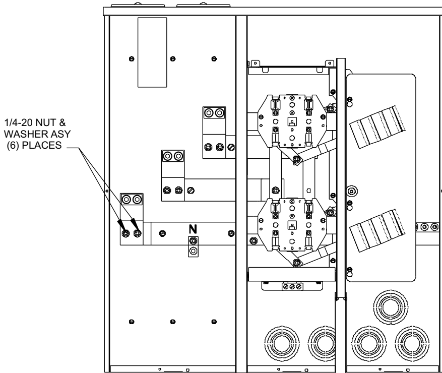
Figure 1 Underground Feed
