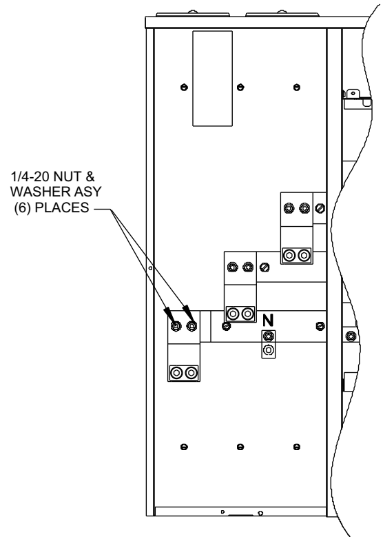
Figure 2 Overhead Feed
