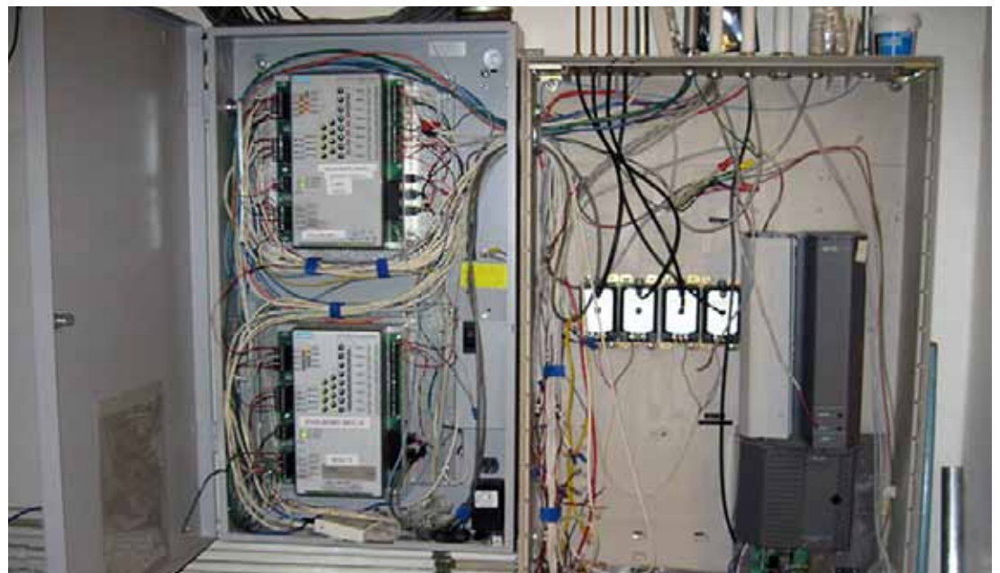
Migrating a JCI panel to Siemens Control panel reusing existing wiring and integrating to remaining JCI N2 devices.
