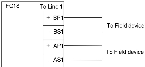
Fig. 2 Field device connection diagram (the same for other line)
