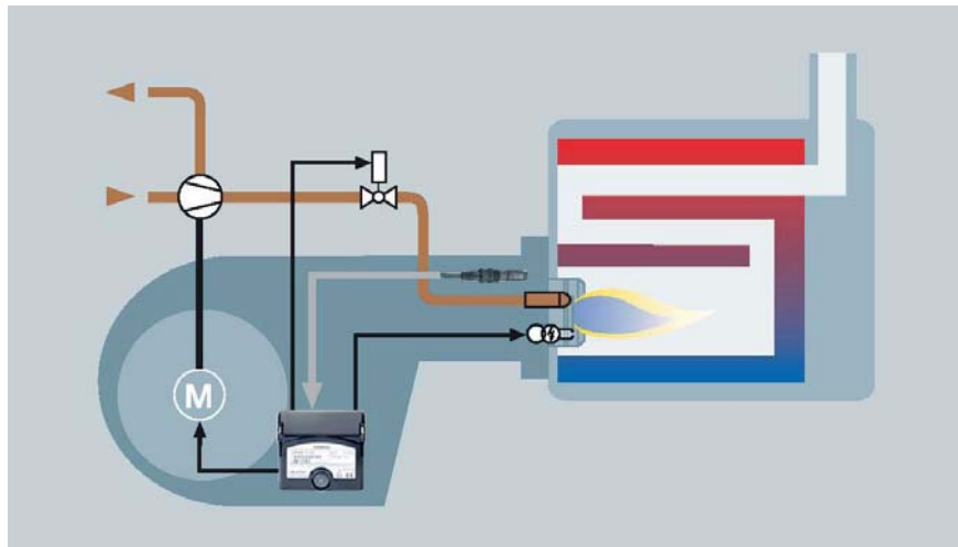
Figure: Overview of the burner system with LMO burner control
