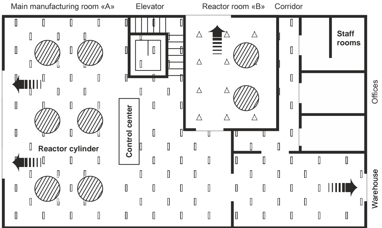
Figure 3: Example of zone classification:
