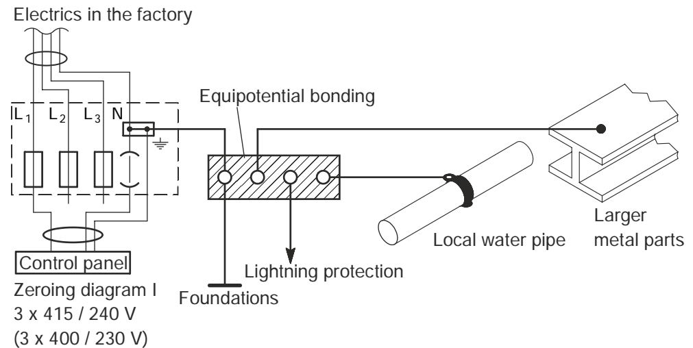
Example of equipotential bonding grounding
