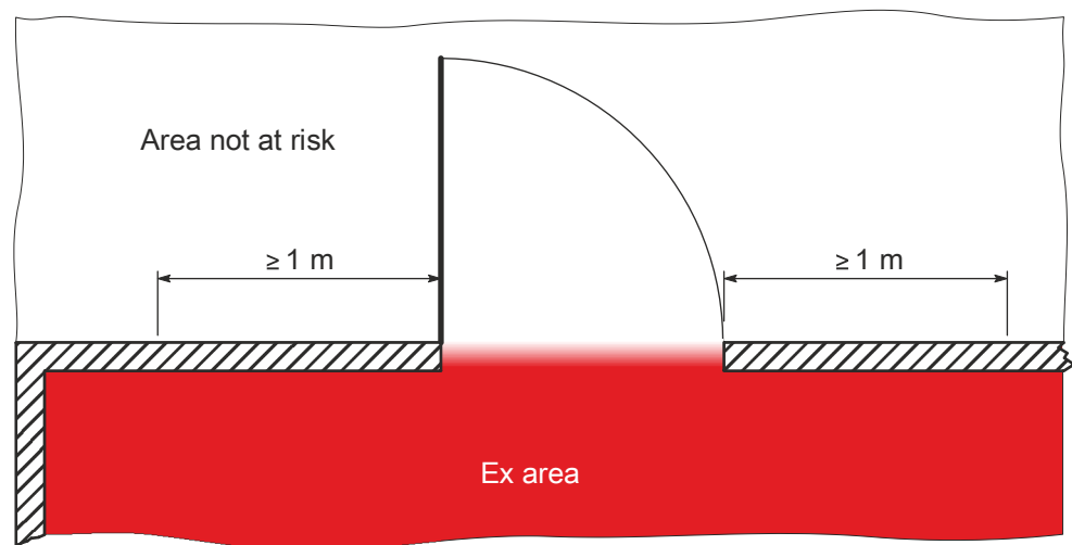
Figure 6: Protective spacing at door and ventilation openings
