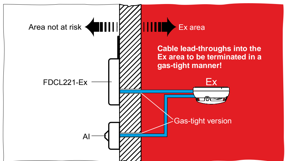
Figure 11: Schematic diagram of the usual arrangement of an external alarm indicator
