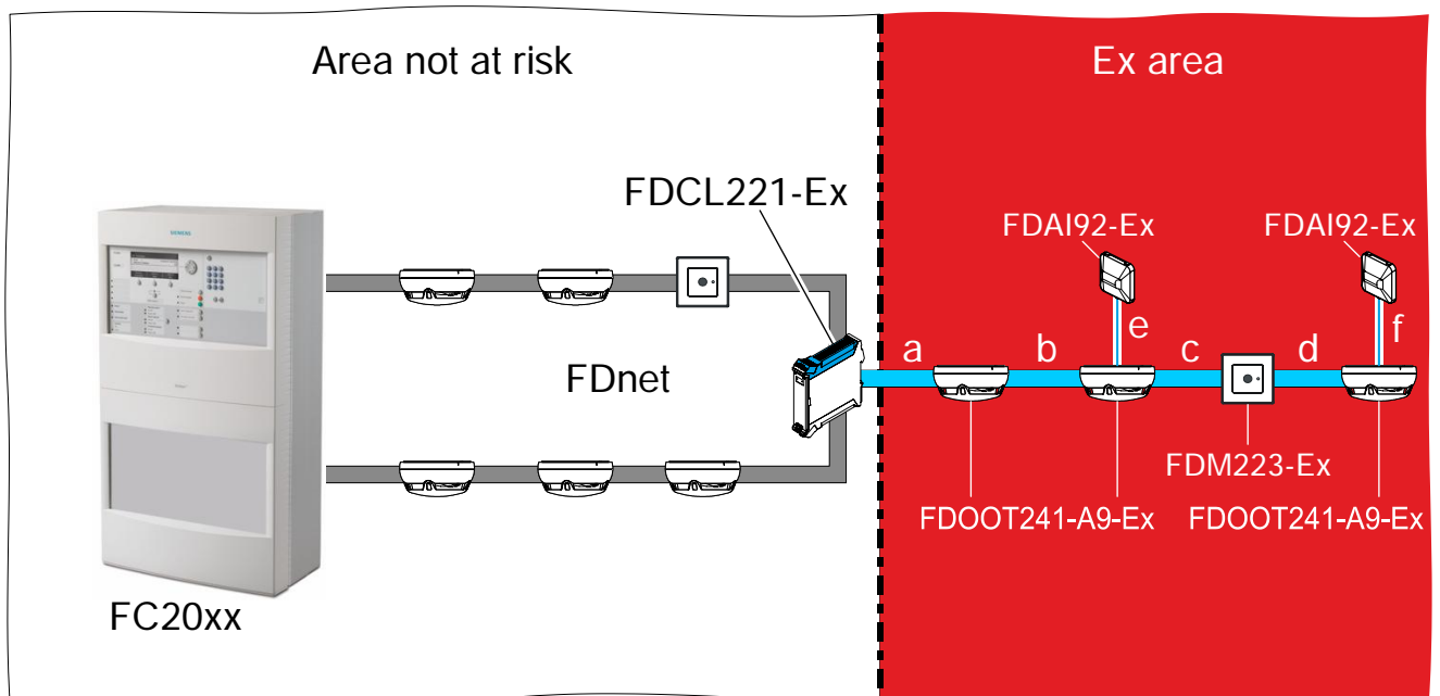
Example of a 'Sinteso' fire detection installation being planned in a potentially explosive atmosphere
