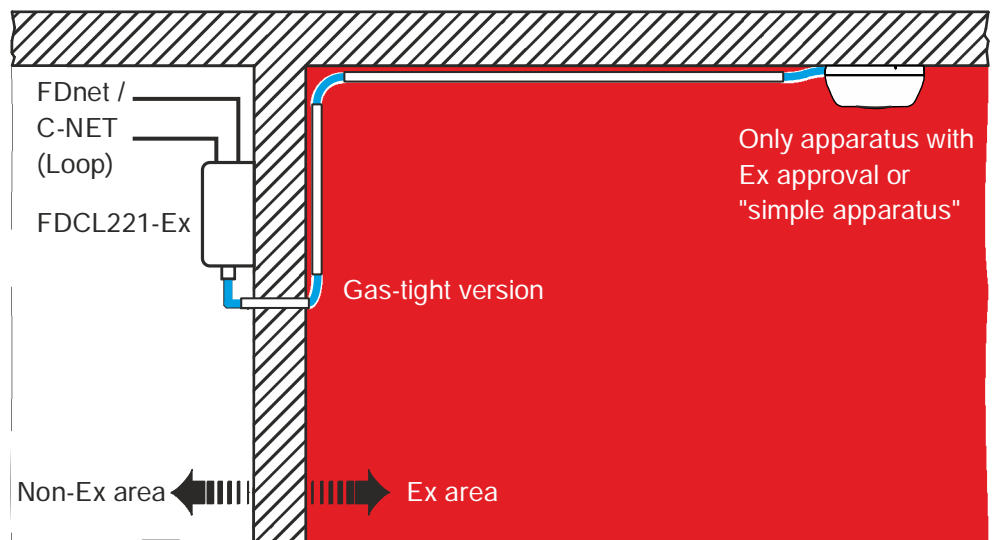
Example of installation in an area at risk of explosion
