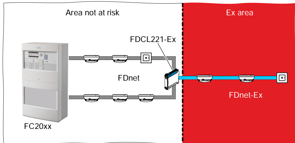
Example of installing a fire detection installation FS20 in an Ex area and a non-hazardous atmosphere
