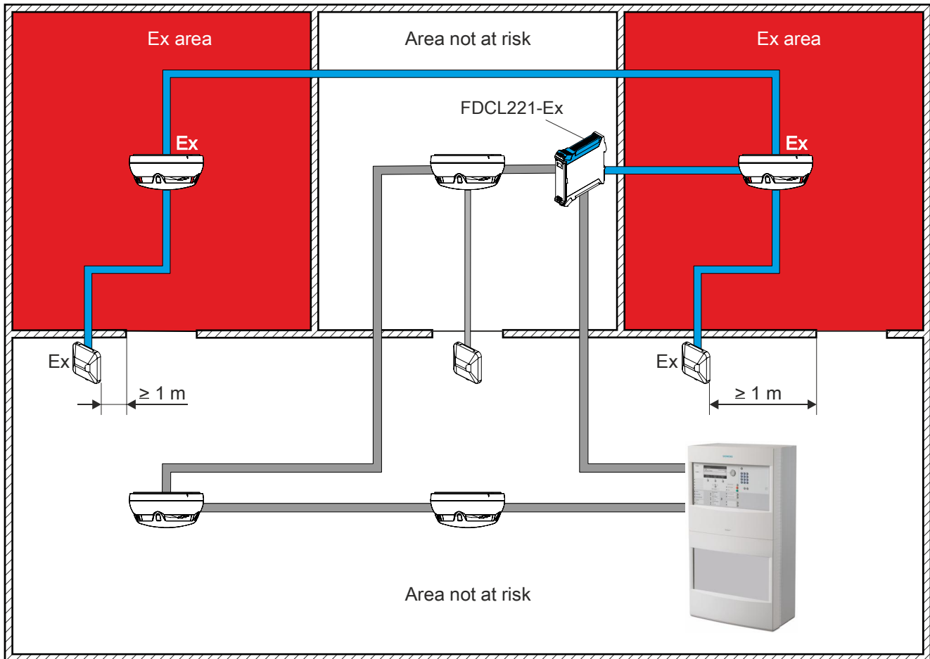
Figure 10: Wiring through non-Ex areas
