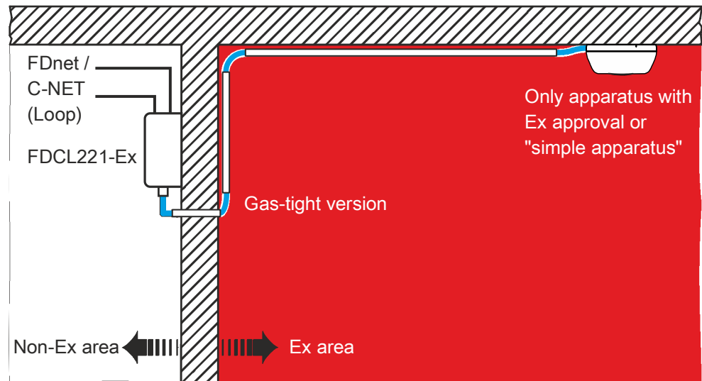
Figure 5: Example of installation in an area at risk of explosion
