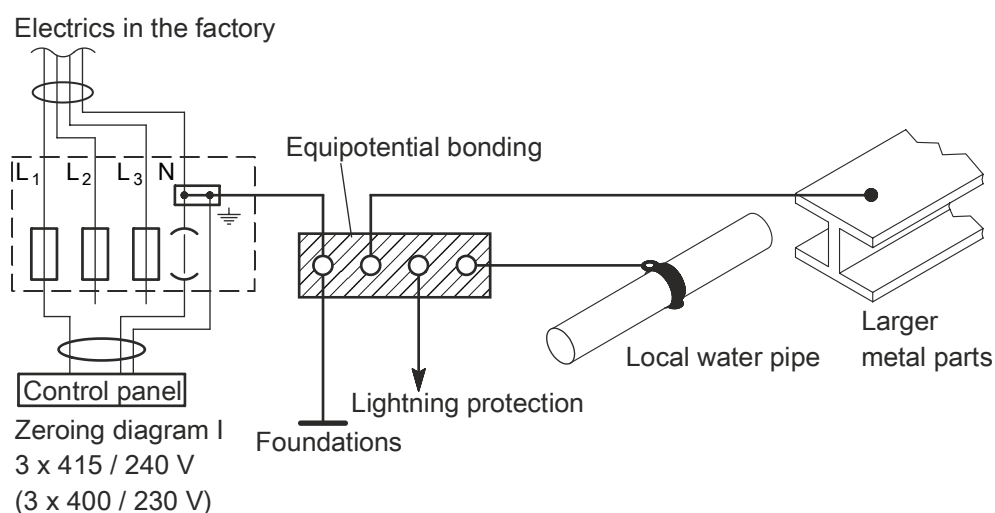
Figure 7: Example of equipotential bonding grounding
