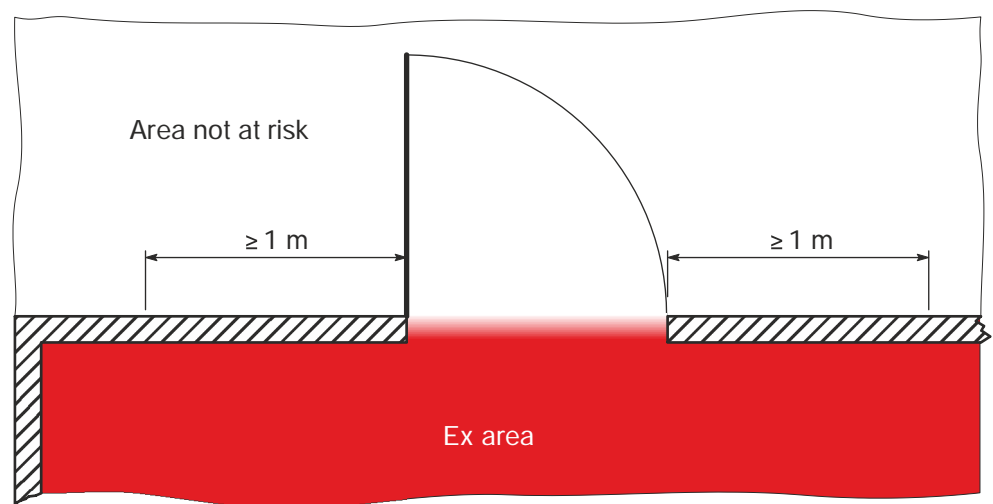
Protective spacing at door and ventilation openings
