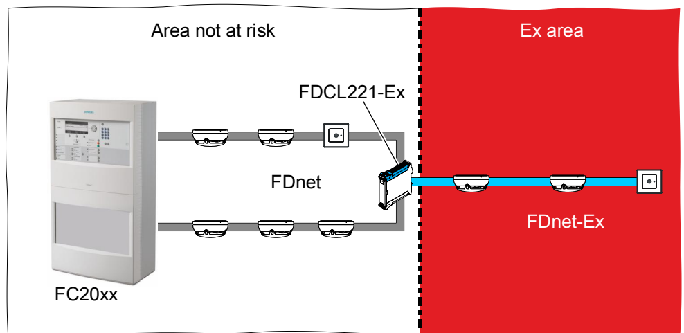
Figure 4: Example of installing a fire detection installation FS20 in an Ex area and a non-hazardous atmosphere
