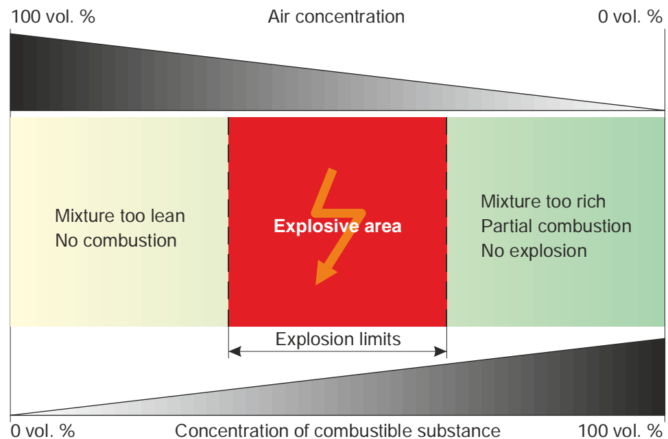
Explosion limits
