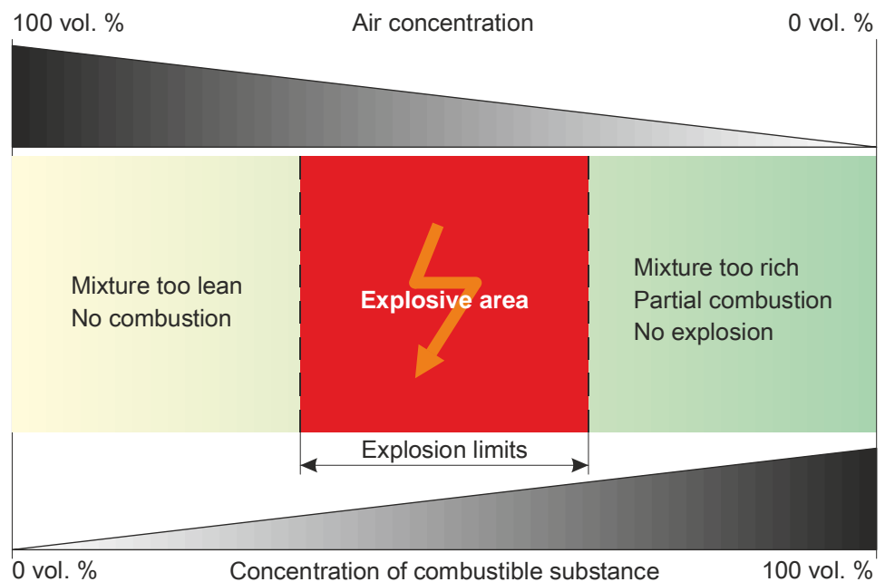
Figure 2: Explosion limits
