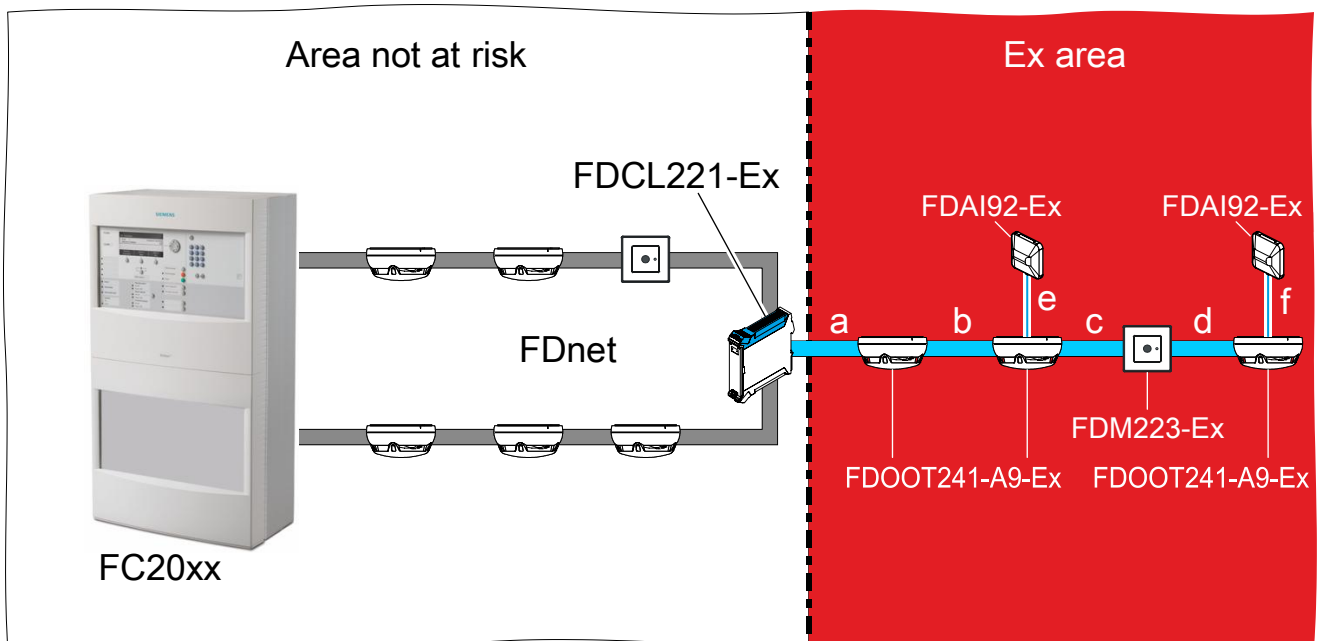
Figure 12: Example of a 'Sinteso' fire detection installation being planned in a potentially explosive atmosphere
