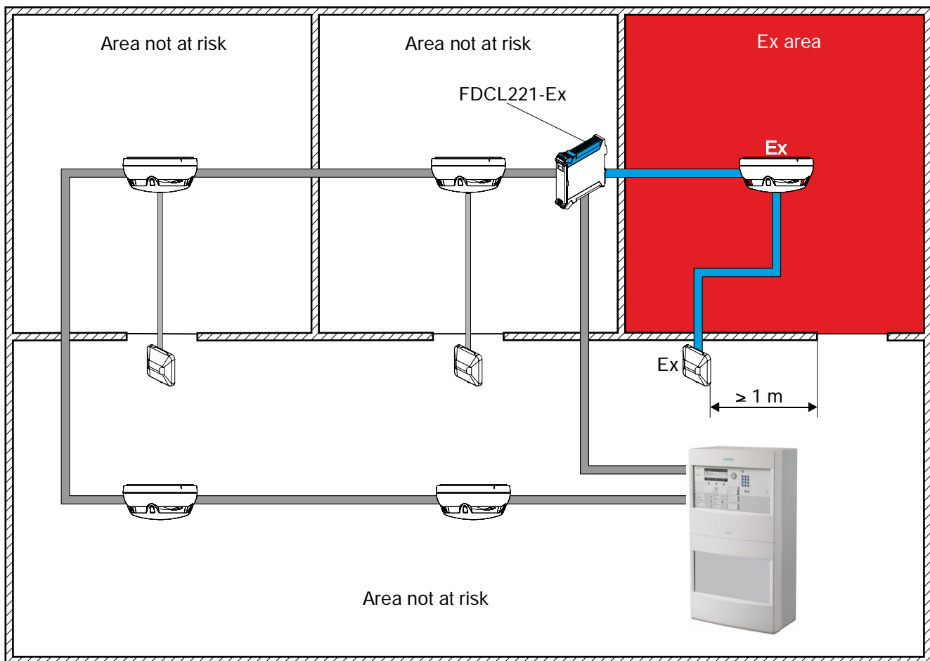
Example of a fire detection installation in an area at risk of explosion
