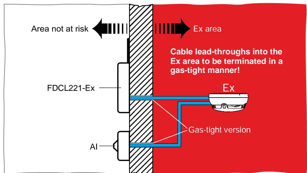
Schematic diagram of the usual arrangement of an external alarm indicator
