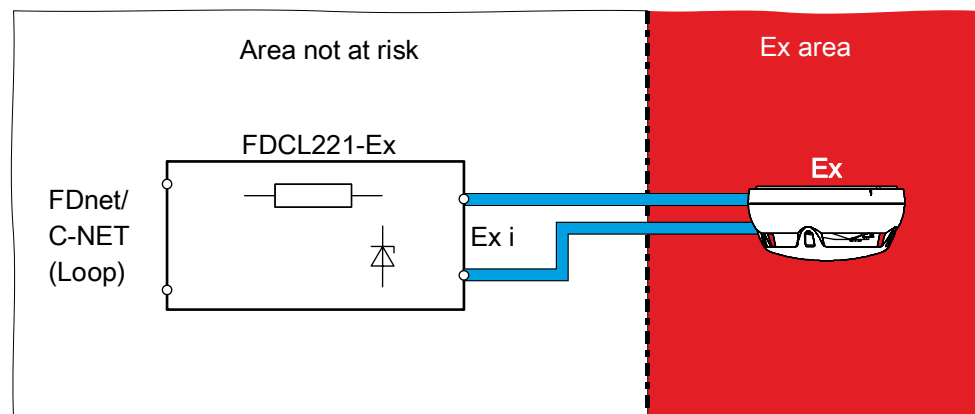
Figure 8: Intrinsically safe circuit with line adapter (Ex) FDCL221-Ex
