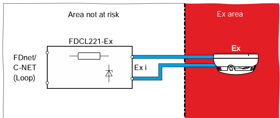
Intrinsically safe circuit with line adapter (Ex) FDCL221-Ex
