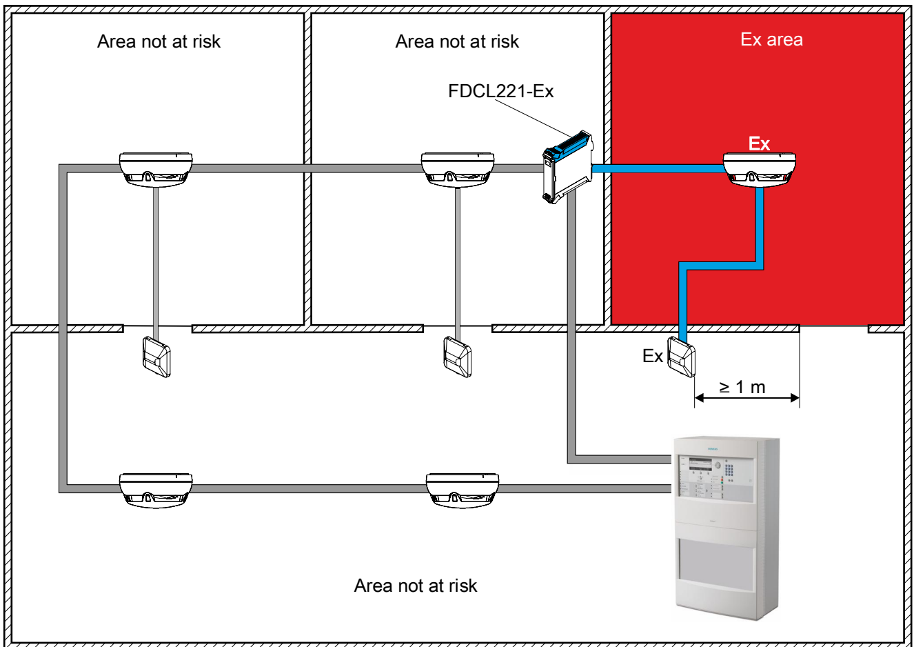
Figure 9: Example of a fire detection installation in an area at risk of explosion
