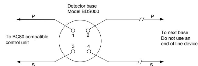
Figure 2 Installation and wiring diagram
