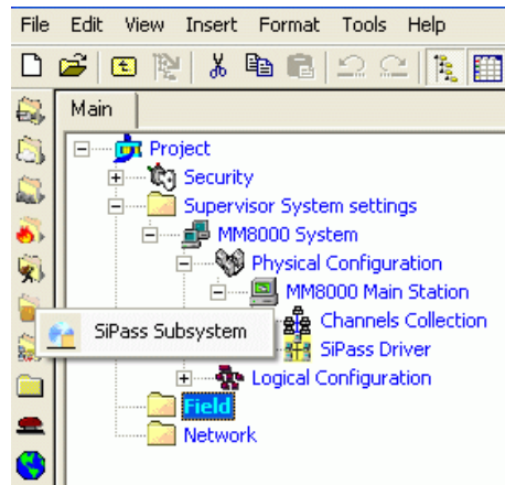
Adding the SiPass subsystem
