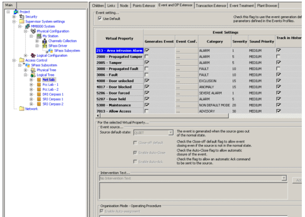
Customising individual SiPass points event settings
