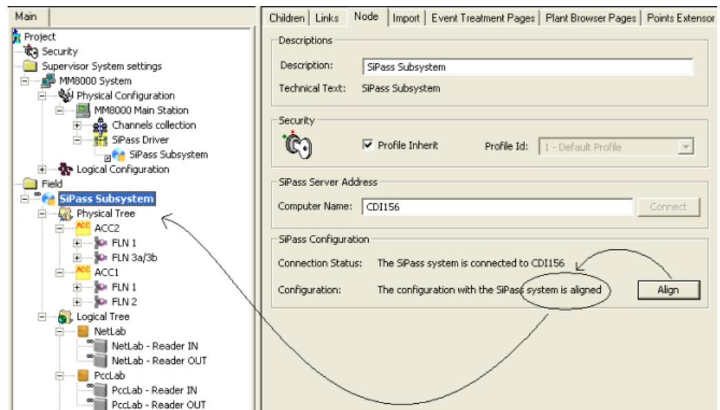
Transferring SiPass configuration
