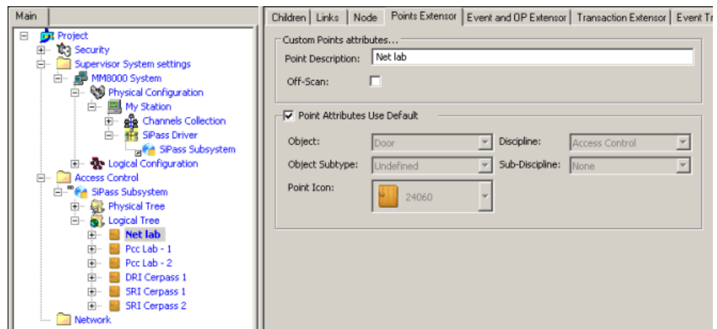
Customising individual SiPass points
