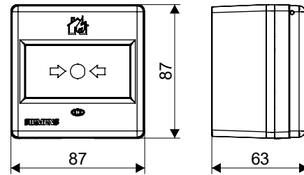
Radio manual call points FDM275 and FDM275(F)
