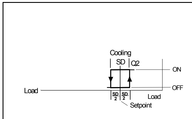
Cooling sequence
