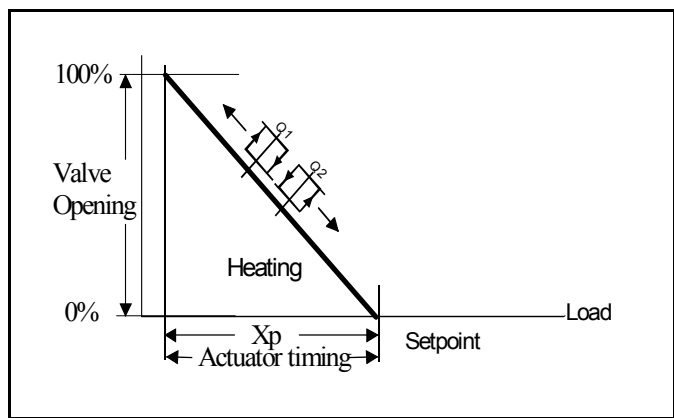
Heating sequences
