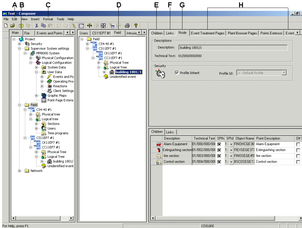
Fig. 2 Split tree example with split data view
