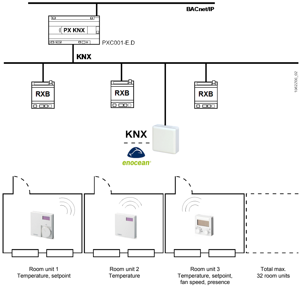
Integration of EnOcean room units in Design RXB and building automation and control systems
