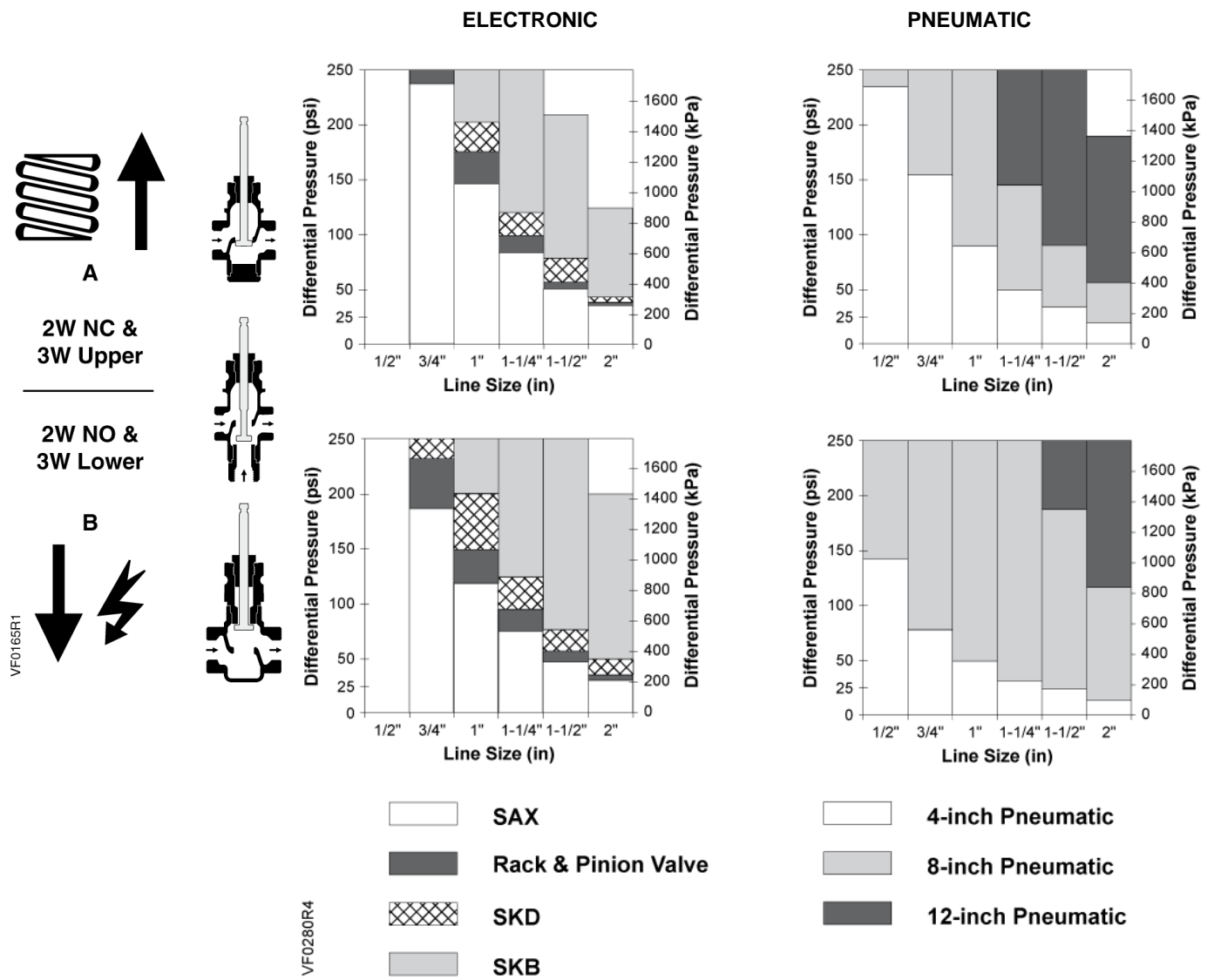
Figure 3. Close-off Pressures.
