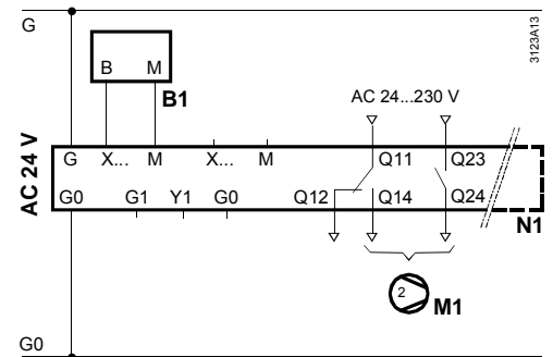
Diagram 5: Connection of a 2-speed fan
