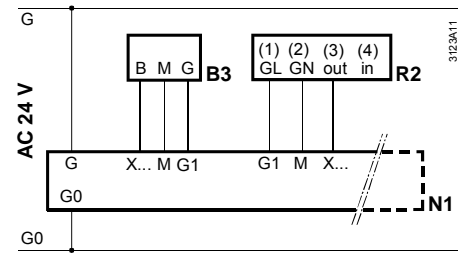
Diagram 2: Measuring section with active sensor and signal source
