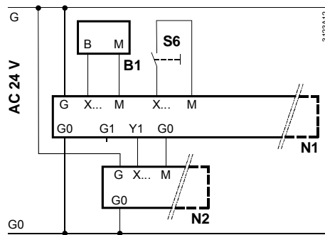
Diagram 4: Multiple use of sensors (B1, N2), external changeover of operating mode (S6)
