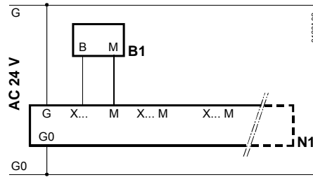
Diagram 1: Measuring section with passive sensor
