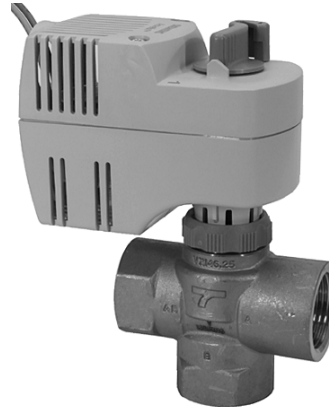
3-port valve MXI421.15 to MXI421.25
